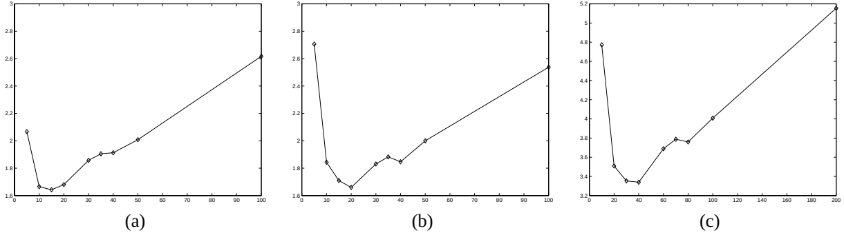
Figure 4: Determining codebook size for edge direction coherence vectors; (a) city class; (b) landscape class; (c) city and landscape classes combined; x-axis represents the codebook size and y-axis represents the optimality criterion to be minimized.
